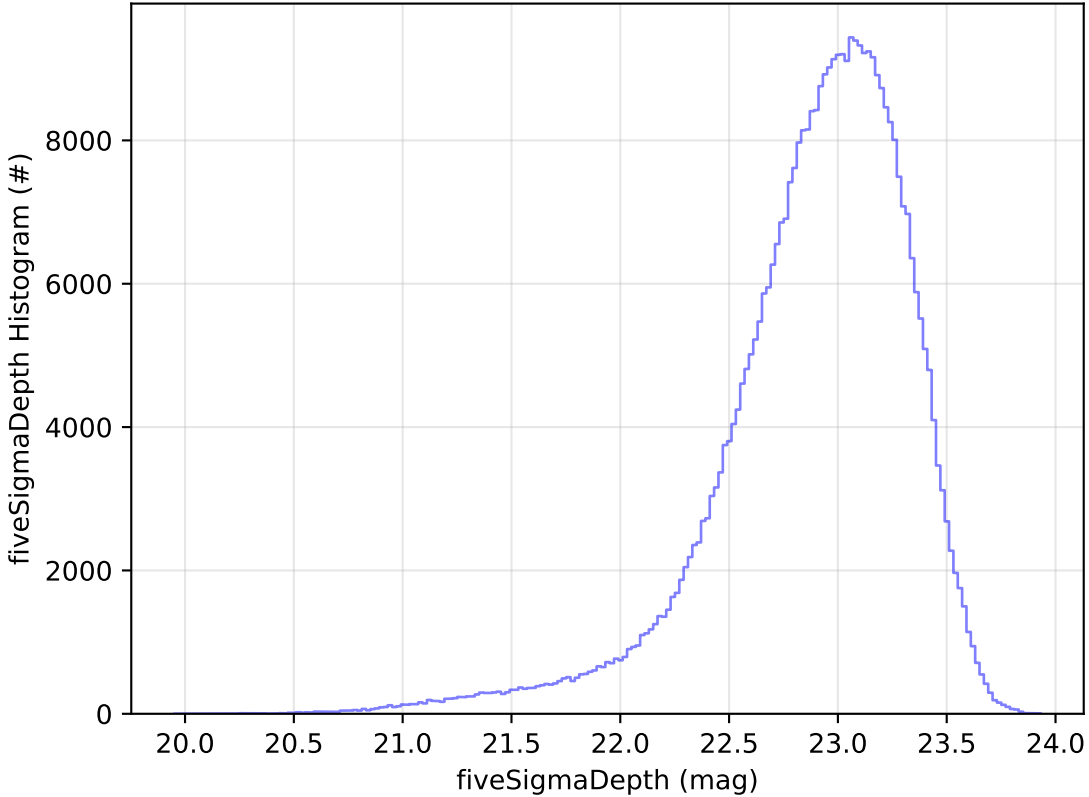
too_elab_r128_d2_gz_v3.4_10yrs All sky z band: fiveSigmaDepth Histogram
