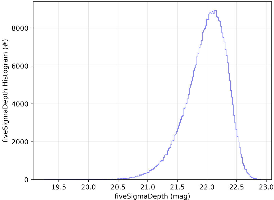
too_elab_r128_d2_gz_v3.4_10yrs All sky y band: fiveSigmaDepth Histogram
