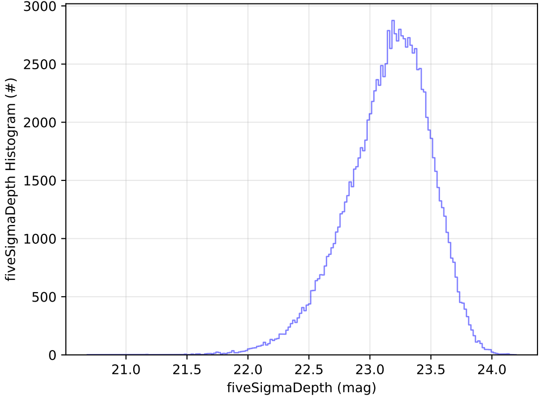
too_elab_r128_d2_gz_v3.4_10yrs All sky u band: fiveSigmaDepth Histogram
