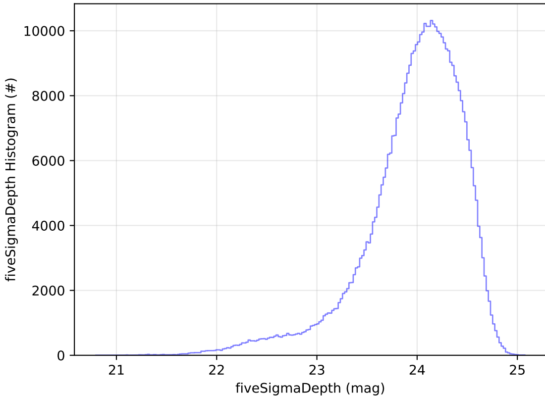
too_elab_r128_d2_gz_v3.4_10yrs All sky r band: fiveSigmaDepth Histogram
