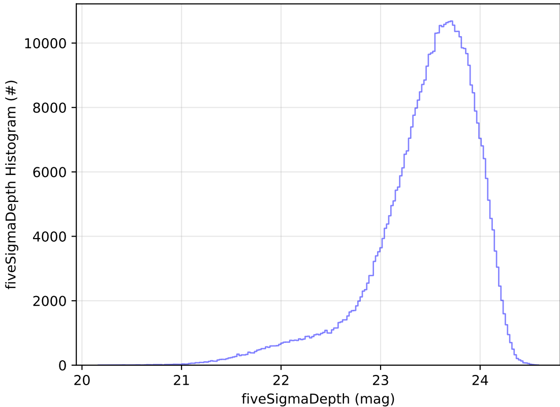
too_elab_r128_d2_gz_v3.4_10yrs All sky i band: fiveSigmaDepth Histogram
