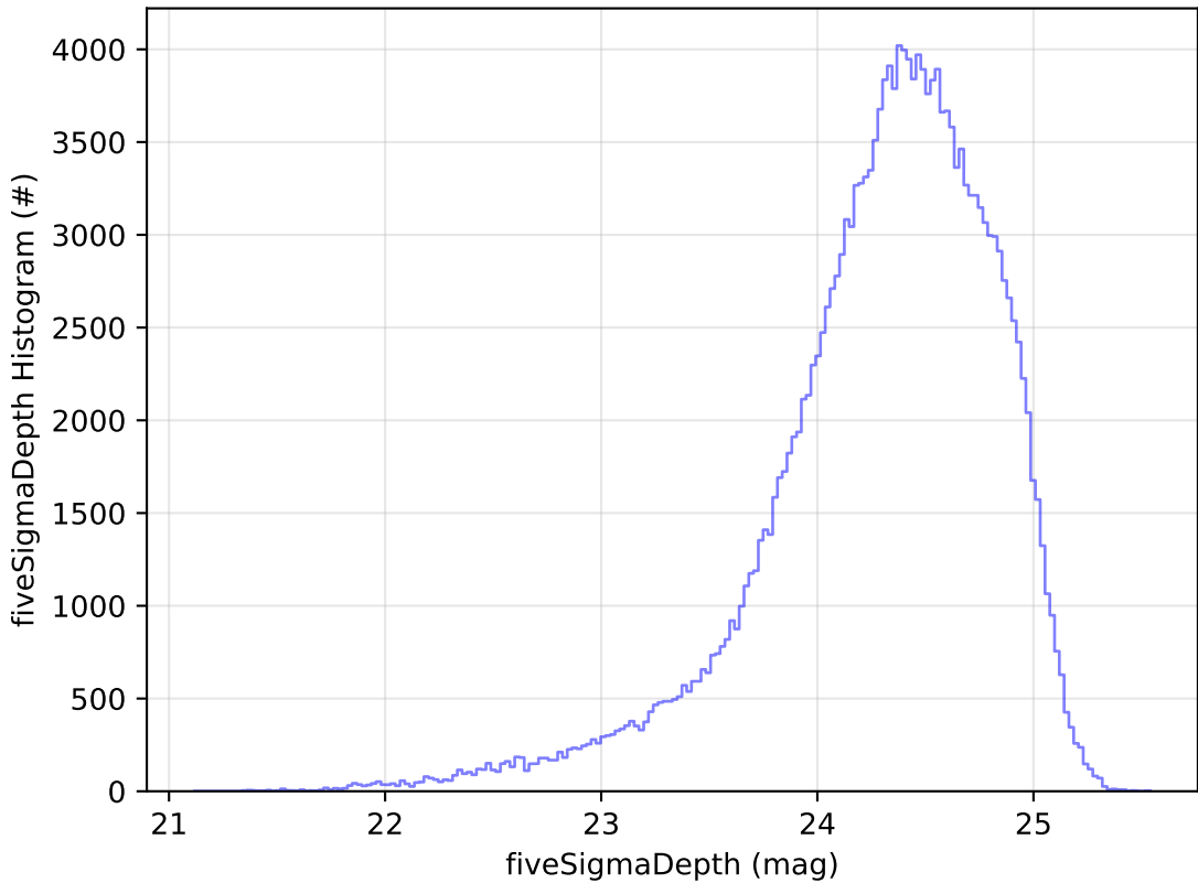
too_elab_r128_d2_gz_v3.4_10yrs All sky g band: fiveSigmaDepth Histogram
