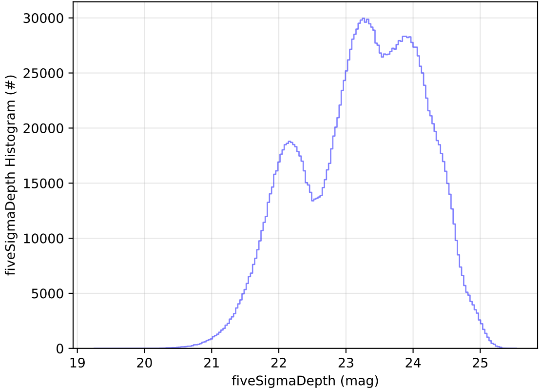
too_elab_r128_d2_gz_v3.4_10yrs All sky all bands: fiveSigmaDepth Histogram
