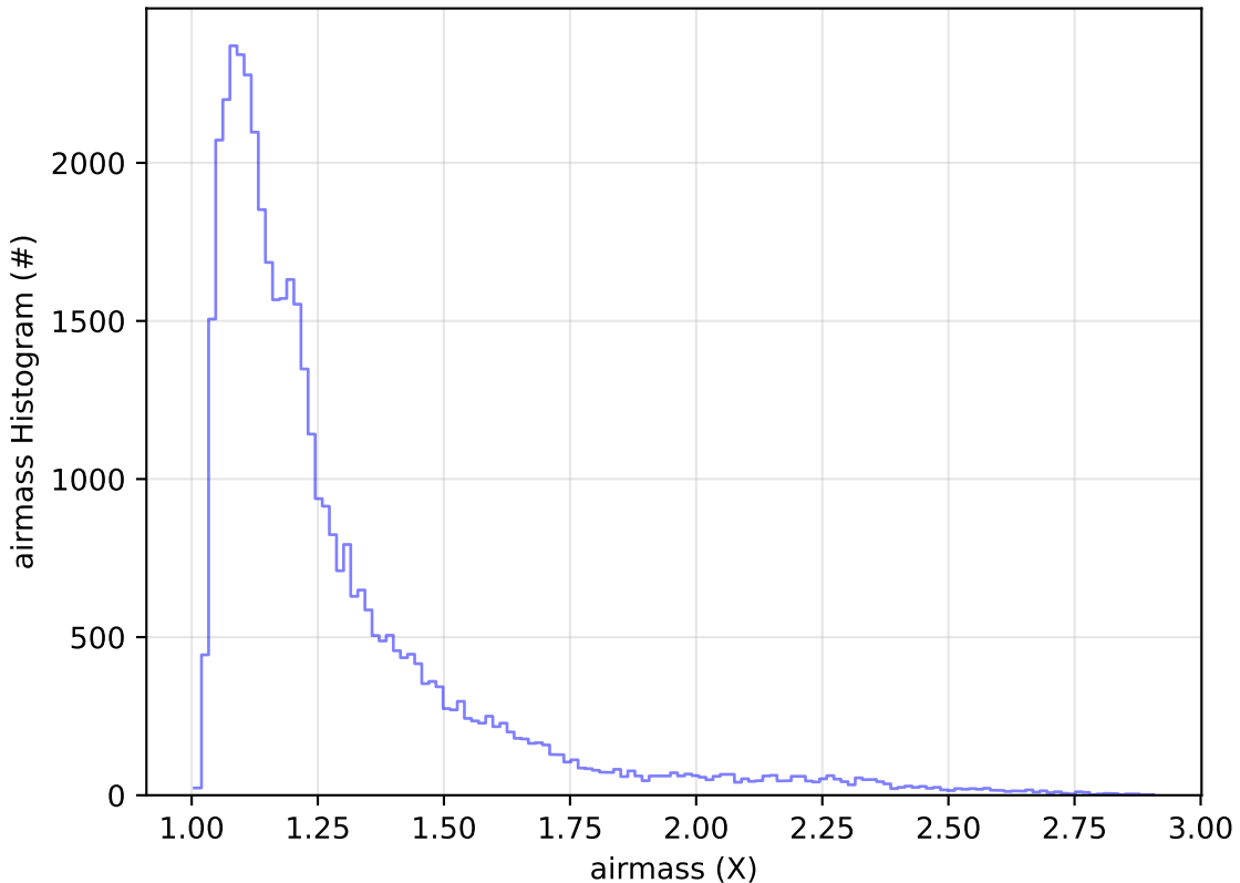
too_elab_r128_d2_gz_v3.4_10yrs Yr 1 z band: airmass Histogram
