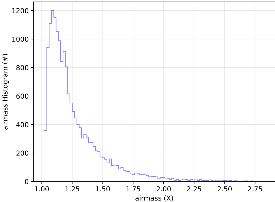
too_elab_r128_d2_gz_v3.4_10yrs Yr 1 u band: airmass Histogram
