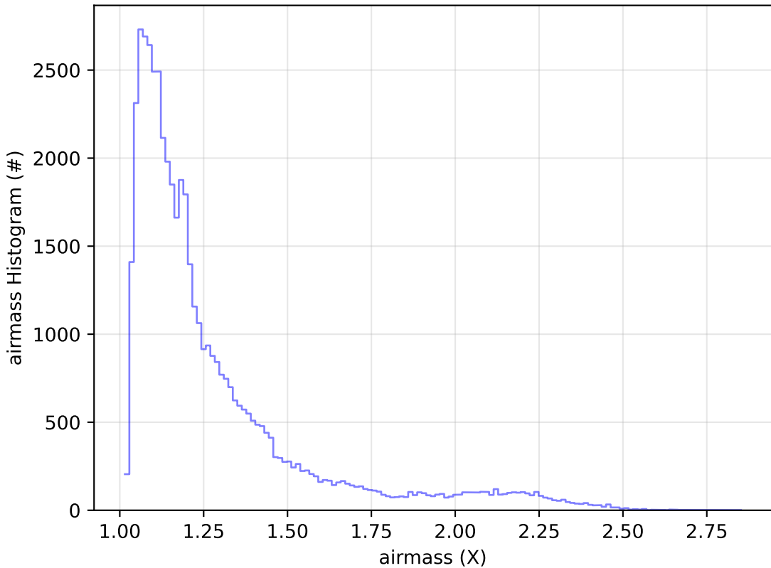
too_elab_r128_d2_gz_v3.4_10yrs Yr 1 r band: airmass Histogram
