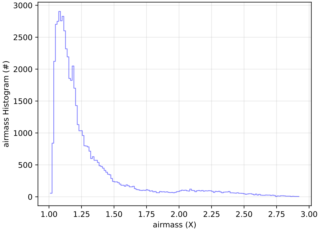
too_elab_r128_d2_gz_v3.4_10yrs Yr 1 i band: airmass Histogram
