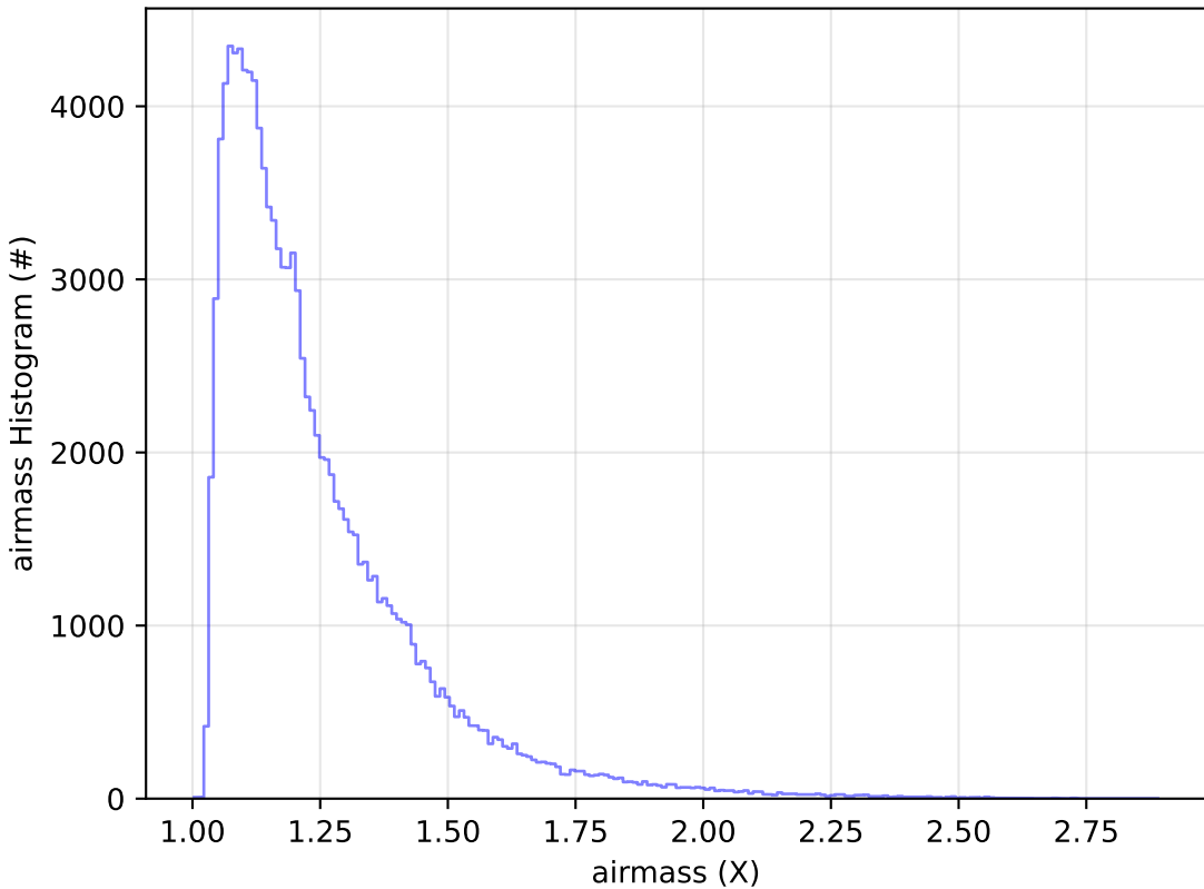
too_elab_r128_d2_gz_v3.4_10yrs WFD u band: airmass Histogram
