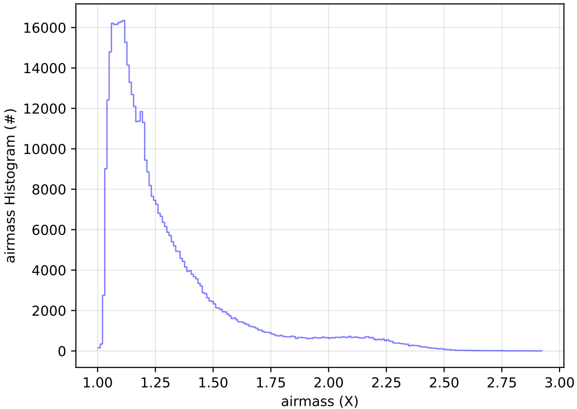
too_elab_r128_d2_gz_v3.4_10yrs WFD r band: airmass Histogram
