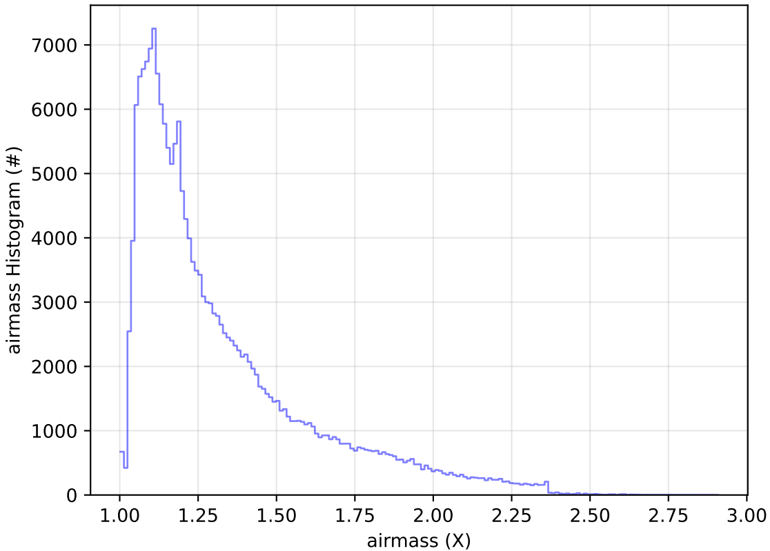
too_elab_r128_d2_gz_v3.4_10yrs WFD g band: airmass Histogram
