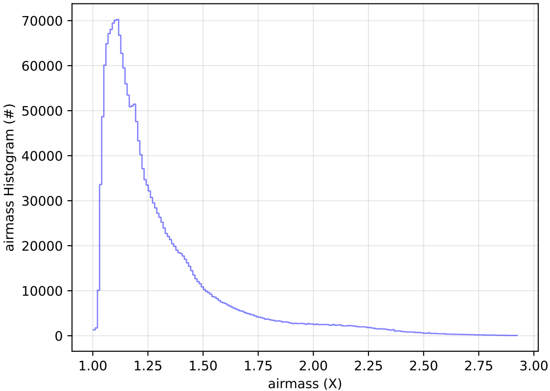
too_elab_r128_d2_gz_v3.4_10yrs WFD all bands: airmass Histogram
