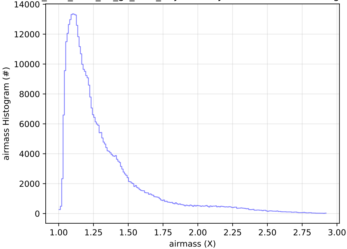
too_elab_r128_d2_gz_v3.4_10yrs All sky z band: airmass Histogram
