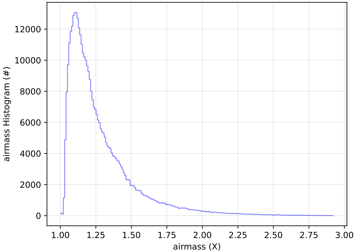
too_elab_r128_d2_gz_v3.4_10yrs All sky y band: airmass Histogram
