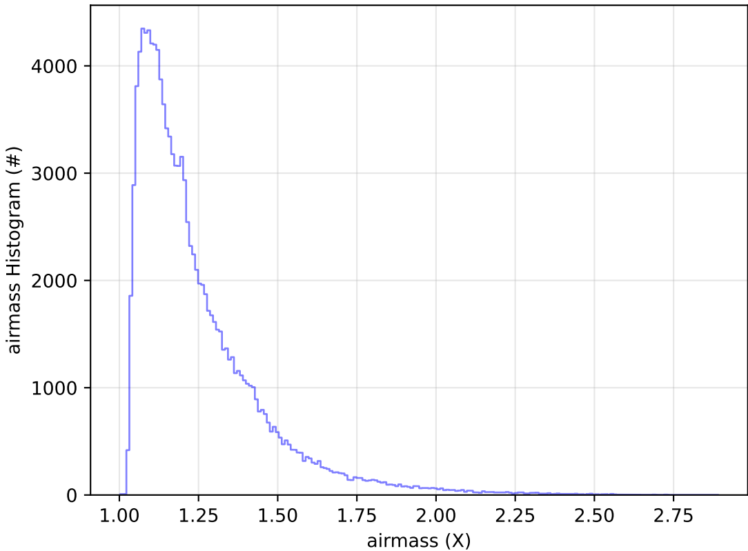
too_elab_r128_d2_gz_v3.4_10yrs All sky u band: airmass Histogram
