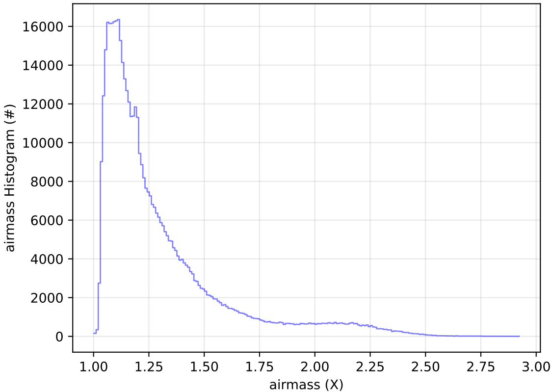
too_elab_r128_d2_gz_v3.4_10yrs All sky r band: airmass Histogram
