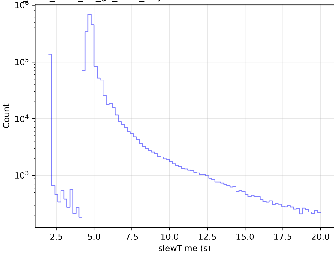
too_elab_r128_d2_gz_v3.4_10yrs All visits: Zoom Slew Time Histogram
