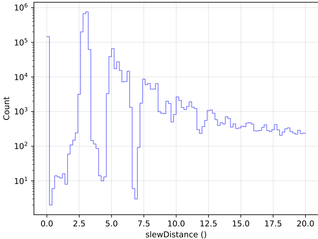
too_elab_r128_d2_gz_v3.4_10yrs All visits: Zoom Slew Distance Histogram
