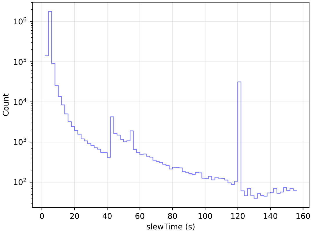
too_elab_r128_d2_gz_v3.4_10yrs All visits: Slew Time Histogram
