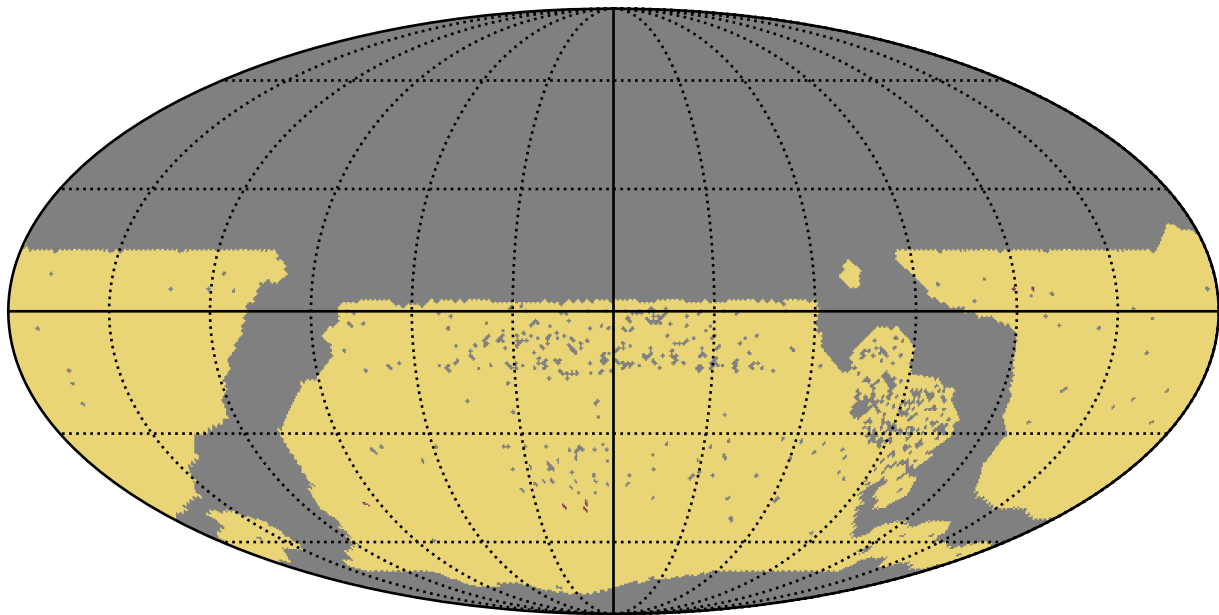
too_elab_r128_d2_gz_v3.4_10yrs WFD: RapidRevisits
