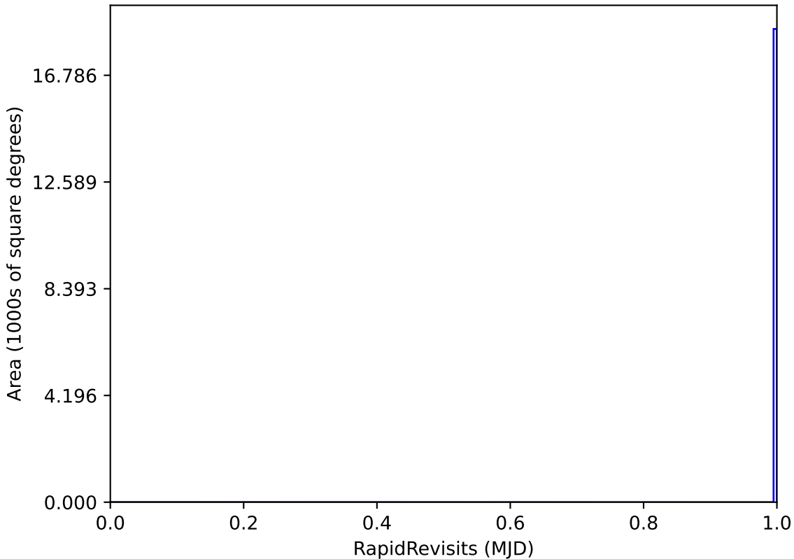
too_elab_r128_d2_gz_v3.4_10yrs WFD: RapidRevisits
