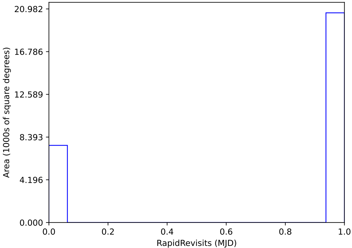
too_elab_r128_d2_gz_v3.4_10yrs All sky: RapidRevisits
