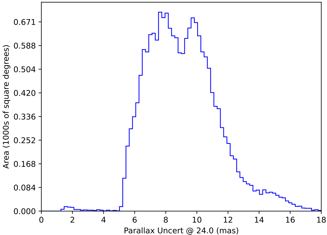
too_elab_r128_d2_gz_v3.4_10yrs WFD: Parallax Uncert @ 24.0
