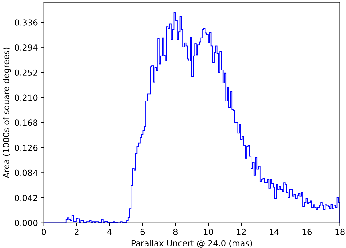
too_elab_r128_d2_gz_v3.4_10yrs All sky: Parallax Uncert @ 24.0
