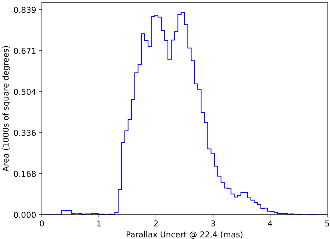
too_elab_r128_d2_gz_v3.4_10yrs WFD: Parallax Uncert @ 22.4
