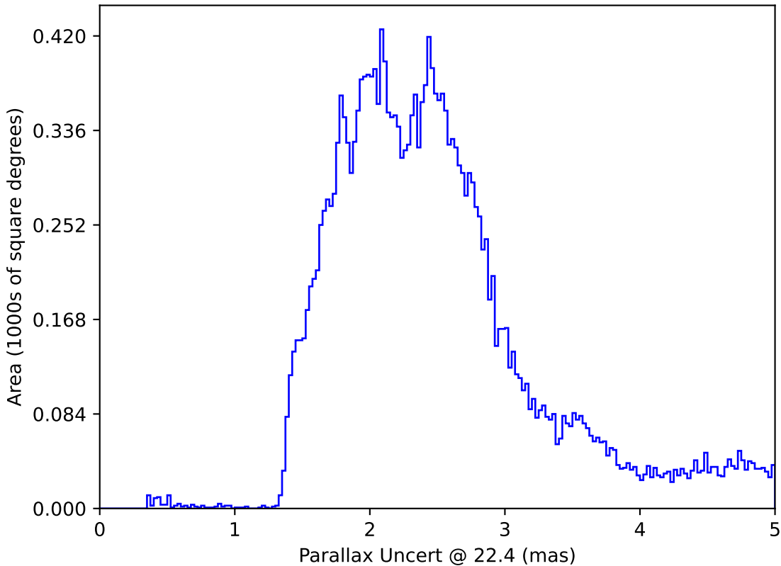
too_elab_r128_d2_gz_v3.4_10yrs All sky: Parallax Uncert @ 22.4
