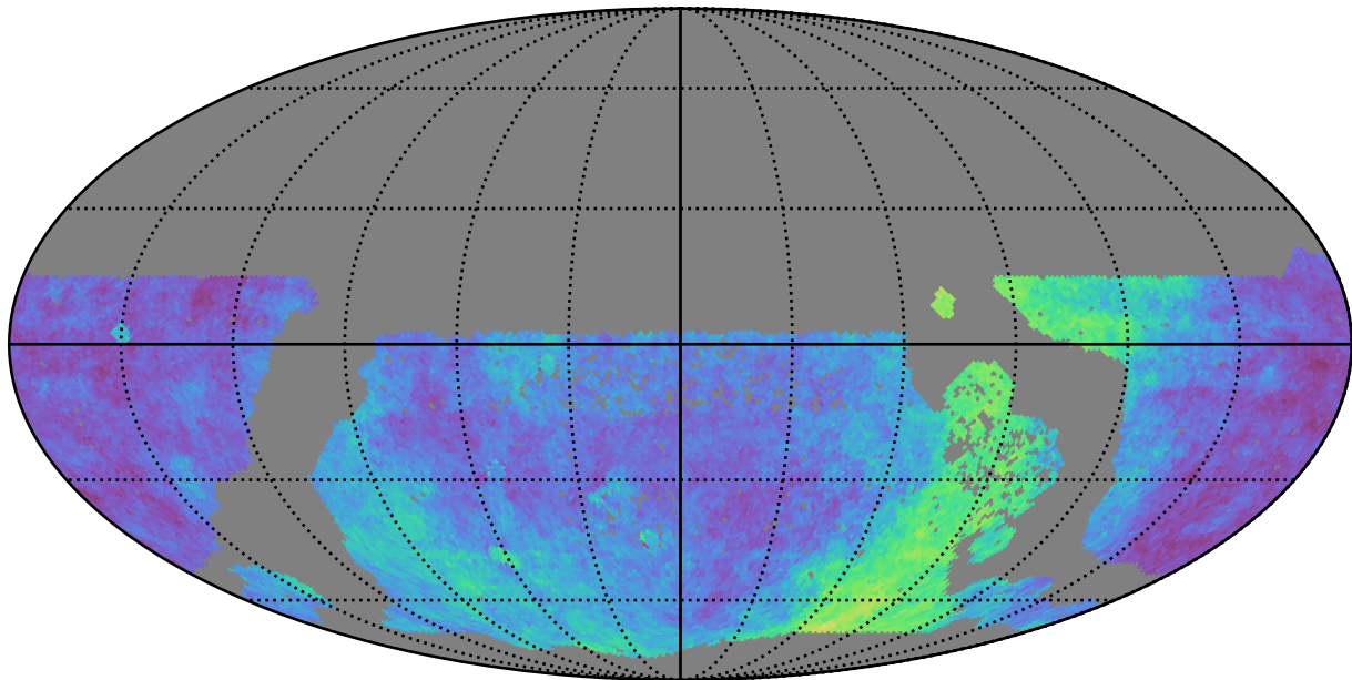
too_elab_r128_d2_gz_v3.4_10yrs WFD: Parallax Coverage @ 24.0
