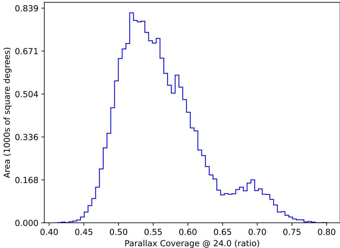
too_elab_r128_d2_gz_v3.4_10yrs WFD: Parallax Coverage @ 24.0
