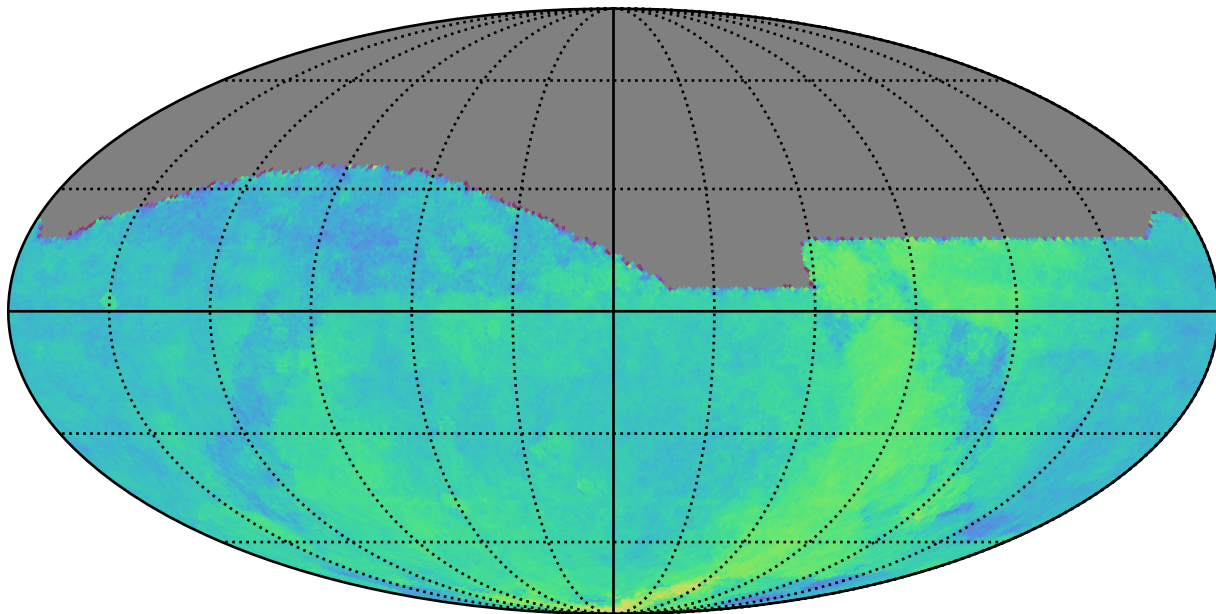
too_elab_r128_d2_gz_v3.4_10yrs All sky: Parallax Coverage @ 24.0
