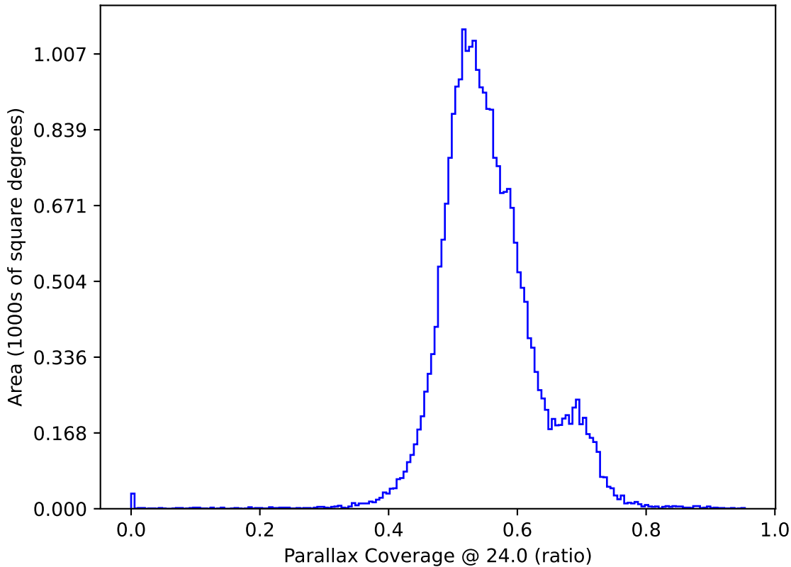
too_elab_r128_d2_gz_v3.4_10yrs All sky: Parallax Coverage @ 24.0
