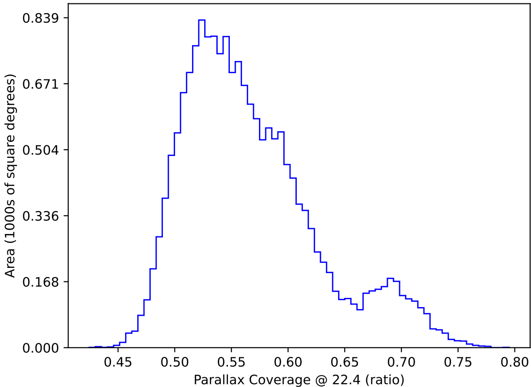
too_elab_r128_d2_gz_v3.4_10yrs WFD: Parallax Coverage @ 22.4
