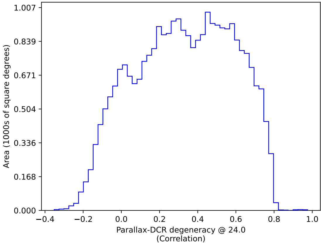
too_elab_r128_d2_gz_v3.4_10yrs All sky: Parallax-DCR degeneracy @ 24.0
