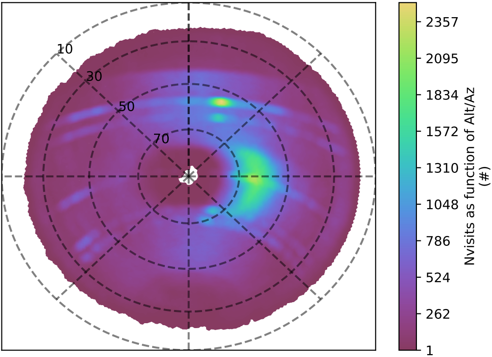
too_elab_r128_d2_gz_v3.4_10yrs z band: Nvisits as function of Alt/Az
