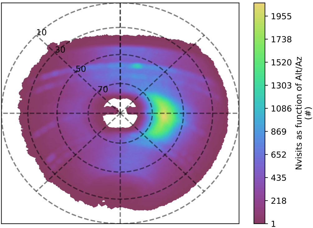
too_elab_r128_d2_gz_v3.4_10yrs y band: Nvisits as function of Alt/Az
