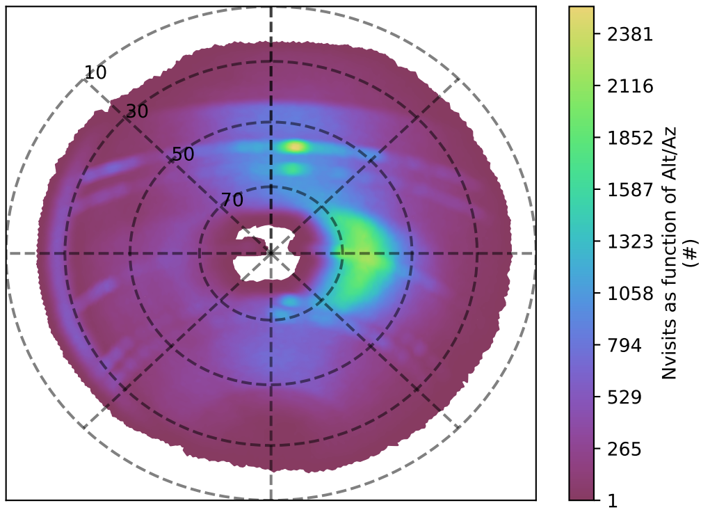
too_elab_r128_d2_gz_v3.4_10yrs r band: Nvisits as function of Alt/Az
