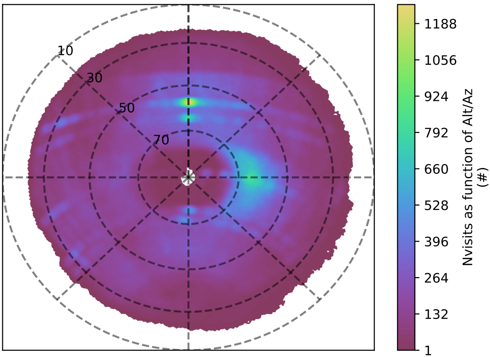
too_elab_r128_d2_gz_v3.4_10yrs g band: Nvisits as function of Alt/Az
