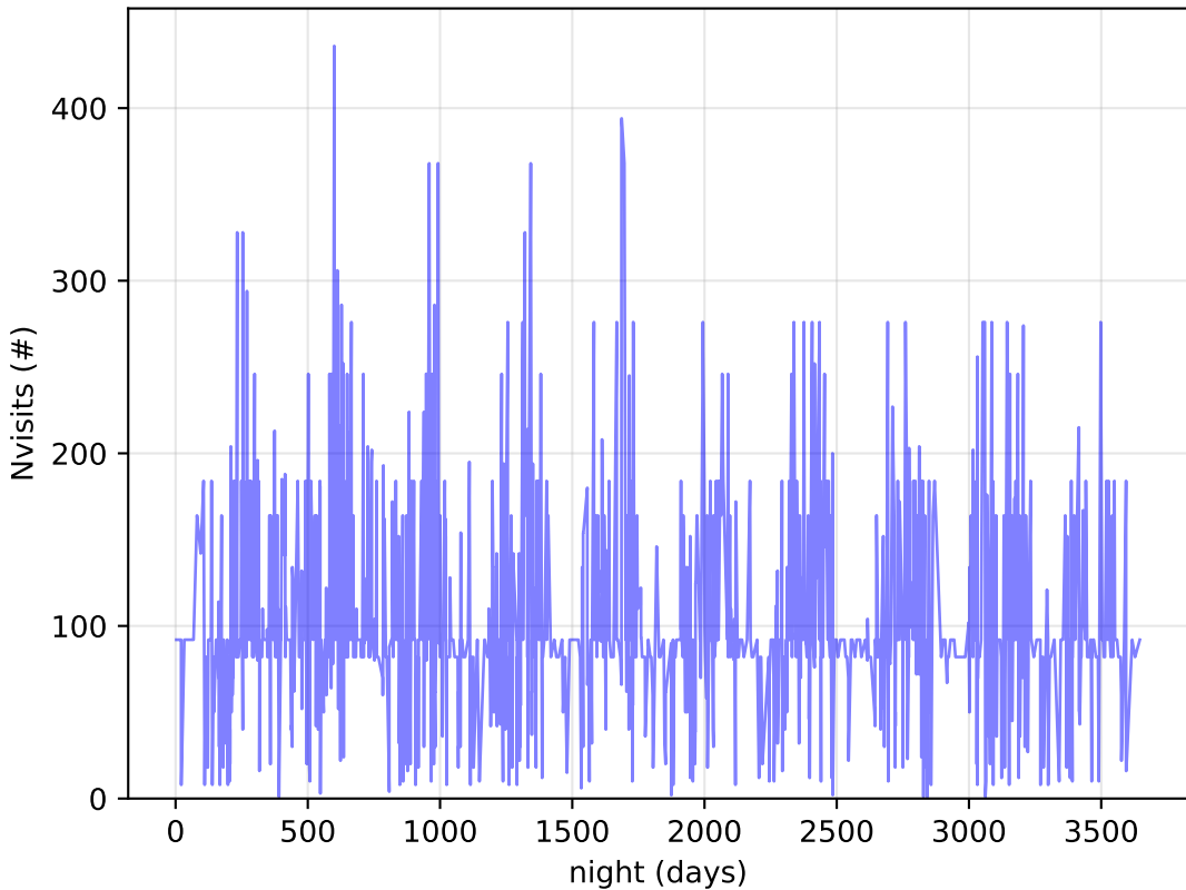
too_elab_r128_d2_gz_v3.4_10yrs DDF: Nvisits
