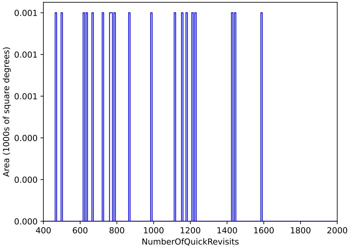
too_elab_r128_d2_gz_v3.4_10yrs WFD: NumberOfQuickRevisits
