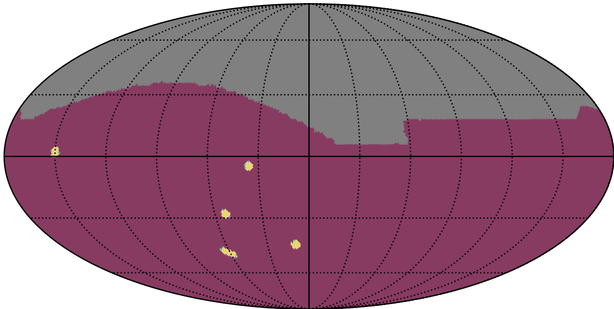
too_elab_r128_d2_gz_v3.4_10yrs All sky: NumberOfQuickRevisits
