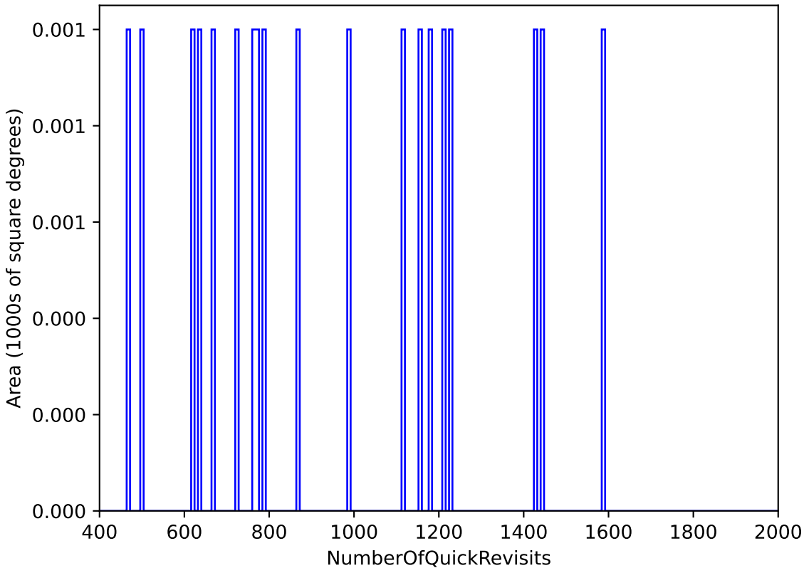
too_elab_r128_d2_gz_v3.4_10yrs All sky: NumberOfQuickRevisits
