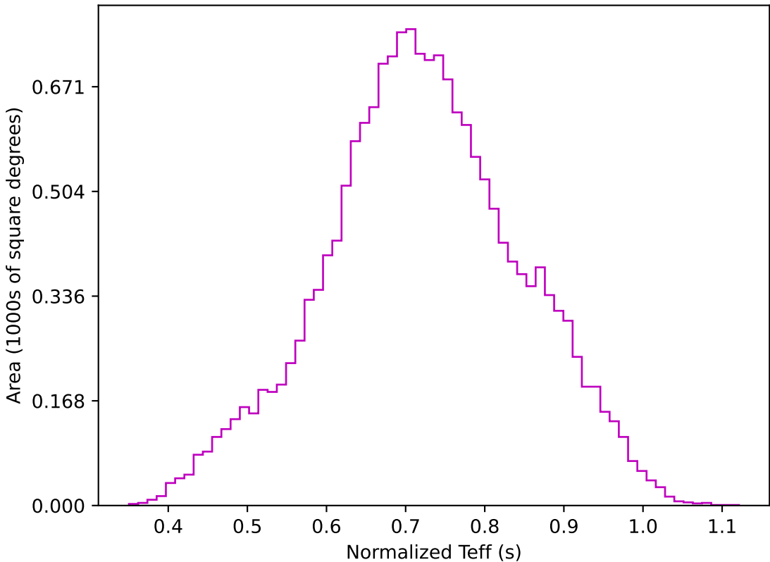
too_elab_r128_d2_gz_v3.4_10yrs WFD z band: Normalized Teff
