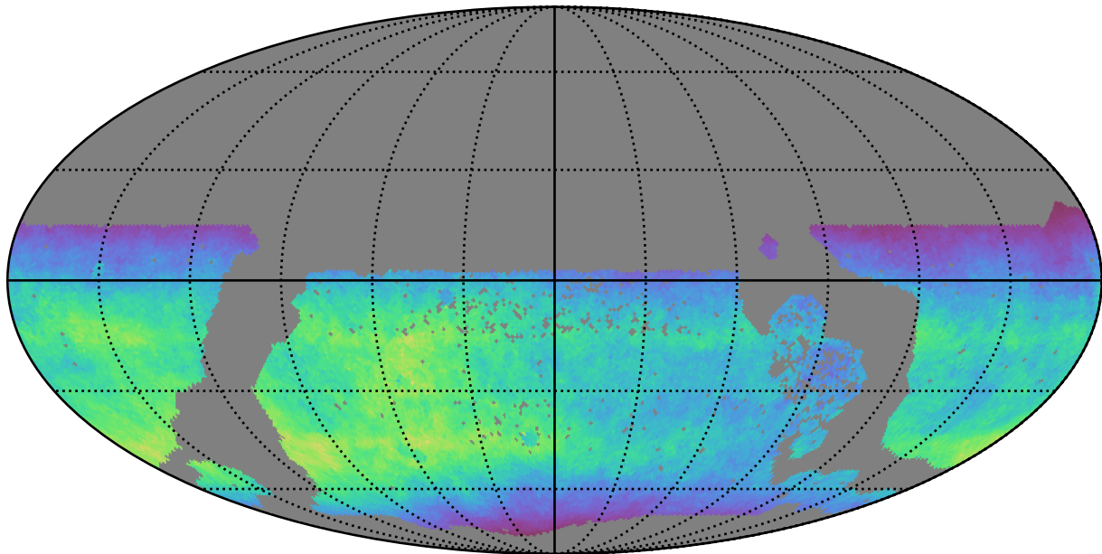
too_elab_r128_d2_gz_v3.4_10yrs WFD y band: Normalized Teff
