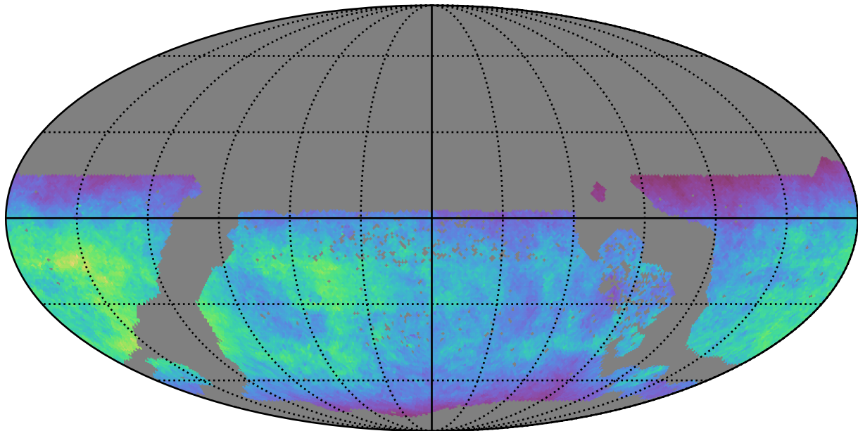
too_elab_r128_d2_gz_v3.4_10yrs WFD u band: Normalized Teff
