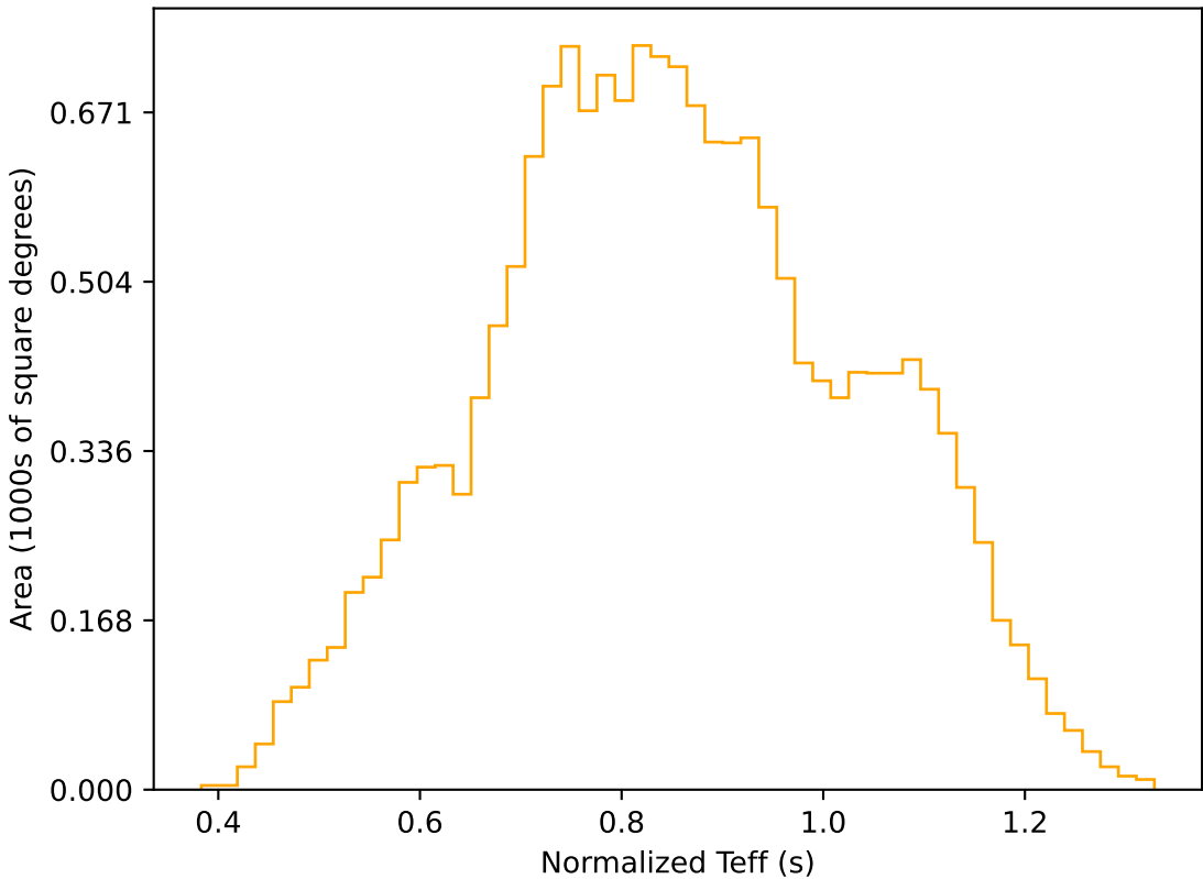
too_elab_r128_d2_gz_v3.4_10yrs WFD r band: Normalized Teff
