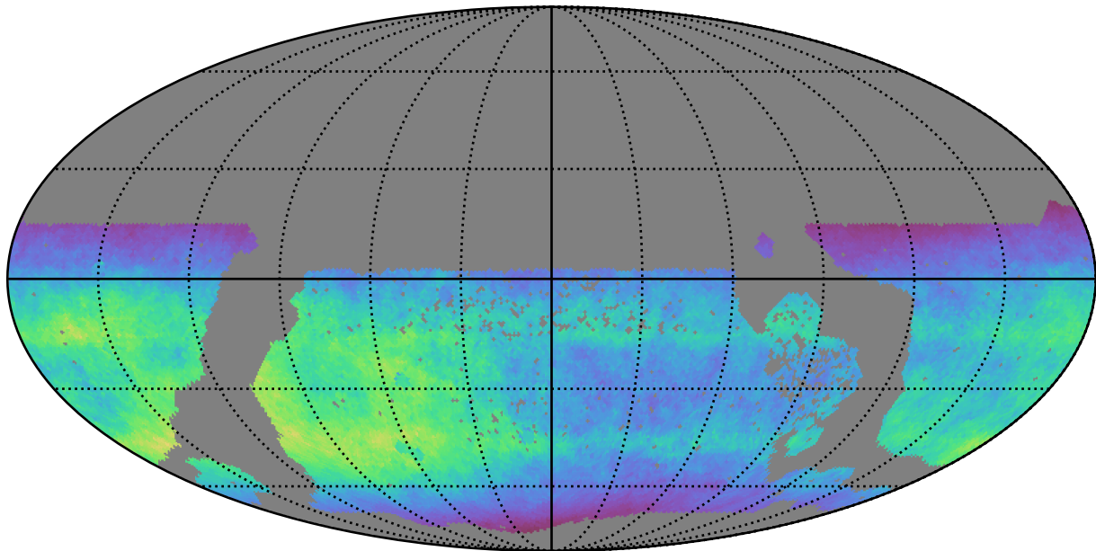
too_elab_r128_d2_gz_v3.4_10yrs WFD i band: Normalized Teff
