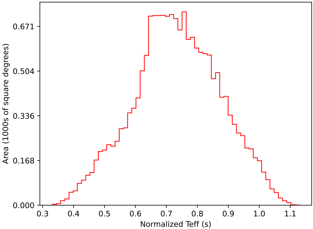
too_elab_r128_d2_gz_v3.4_10yrs WFD i band: Normalized Teff
