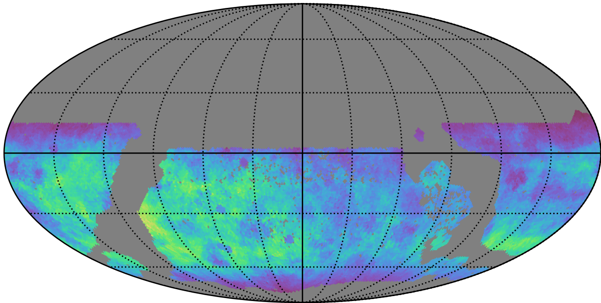
too_elab_r128_d2_gz_v3.4_10yrs WFD g band: Normalized Teff
